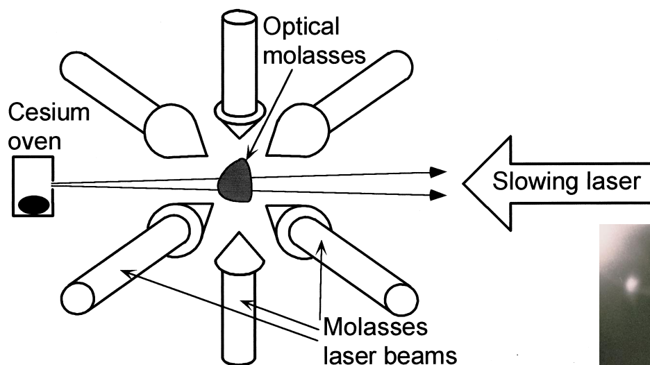
Fig 1 Atoms from a laser-slowed atomic beam are captured in an optical molasses. The molasses, with \sim 10^7 caesium atoms, is formed using 3 pairs of opposing laser beams whose frequency is tuned slightly below the atomic resonance. The damping of the atomic velocities in the molasses is due to a
