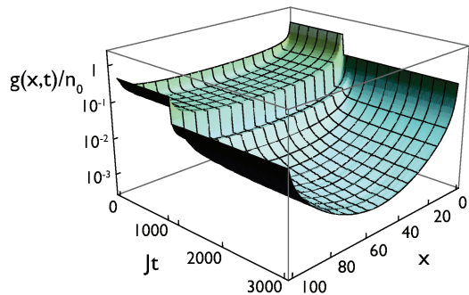
FIG. 5: Single-particle correlation function g(x, t) for \tau_i = 0.89 , for a 100 \times 100 lattice.
