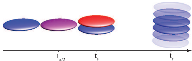
FIG. 1: We prepare a 2D atom cloud in state 1 (blue), and apply a \pi/2 pulse at t_{\pi/2} . We apply a field gradient at t_s , which separates state 1 and 2 (red) spatially. We release the atoms at time t_r and measure their interference properties.
